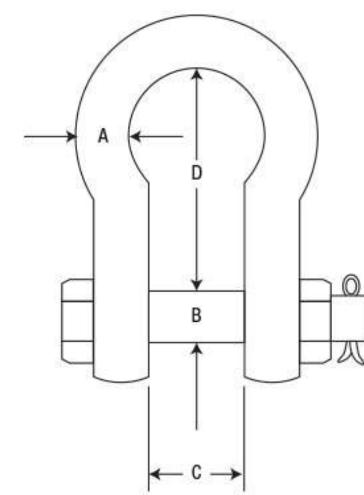
Safety Pin Bow Shackle
